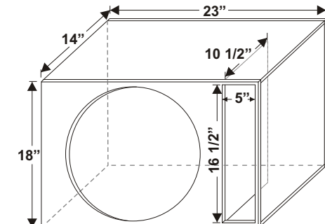
#3 Ported design
